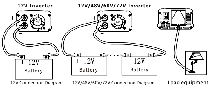
12V Connection Diagram
